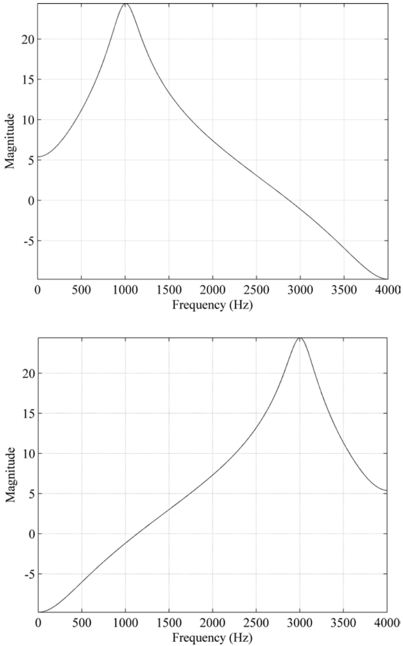
Fig. 3.3. Bi-quad band-pass filter with R_p = 0.90 , f_o = 1 kHz (top) and 3 kHz (bottom).
