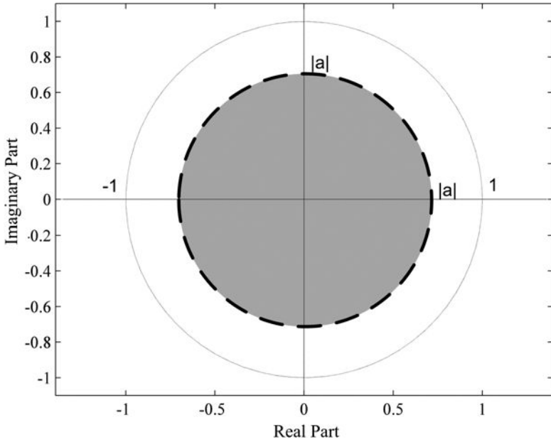
Fig. 5.2. ROC for non-causal h[n] = a^n , |z| < |a| .
