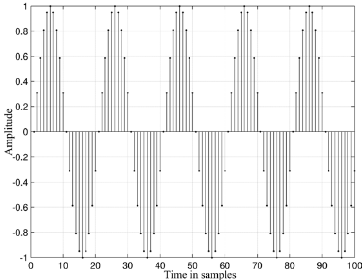
Fig. 4.11. Sine wave at f = 105\text{ Hz} and f_s = 100\text{ Hz} .
