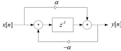
Fig. 3.32. 1st order all pass filter system diagram.
