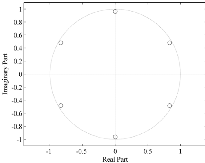
Fig. 3.10. Zero locations for FIR comb-filter with b_1 = 0.8 and L = 6 .
