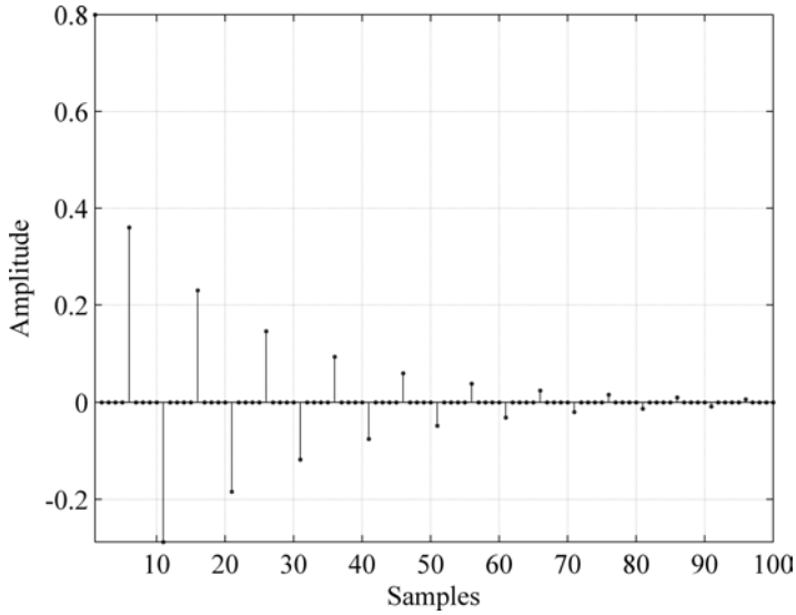
Fig. 3.40. All-pass filter N = 4 , \alpha = 0.8 .
