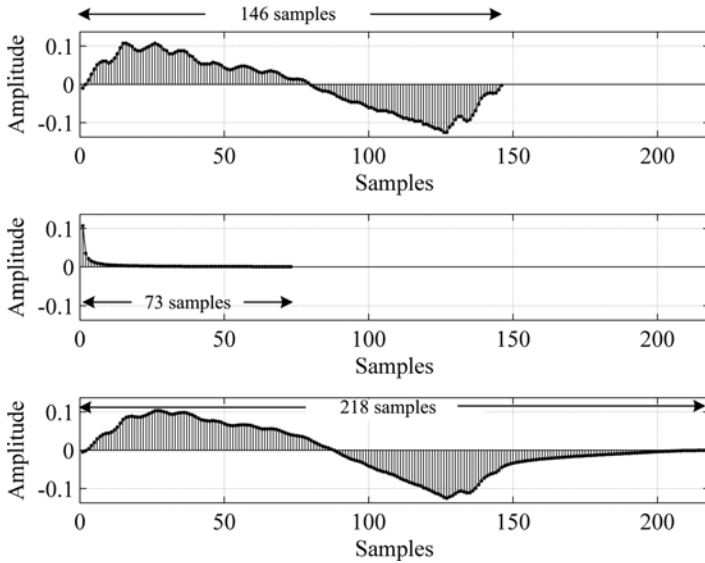
Fig. 11.1. Input signal (top), impulse (middle), and convolution output (bottom).
