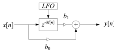
Fig. 3.30. Flanger filter architecture.
