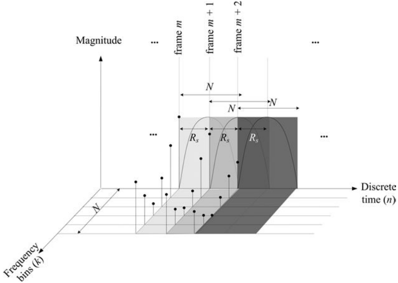
Fig. 3.37. ISTFT model for synthesis in time-shifting.
