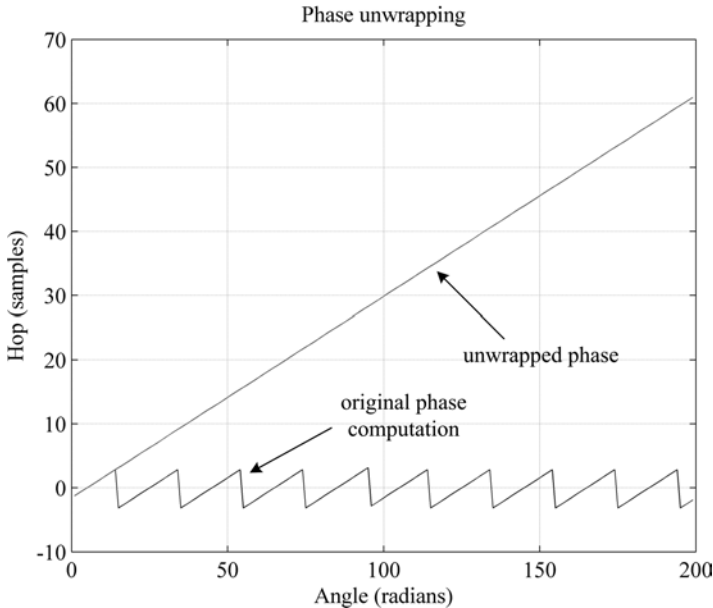
Fig. 3.22. Phase unwrapping.
