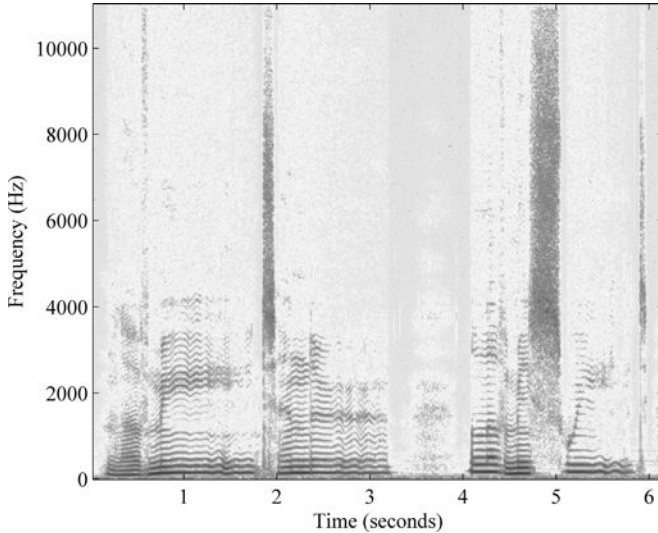
Fig. 13.1. Spectrogram plot.
