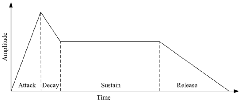
Fig. 2.1. ADSR envelope.
