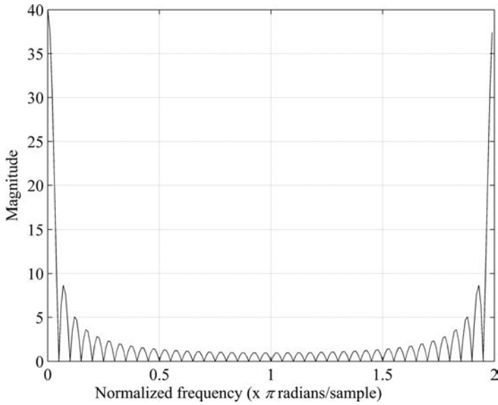
Fig. 9.17. Dirichlet kernel for N = 40 from 0 to 2\pi .
