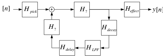
Fig. 3.25. Additional filters for a growing guitar model.
