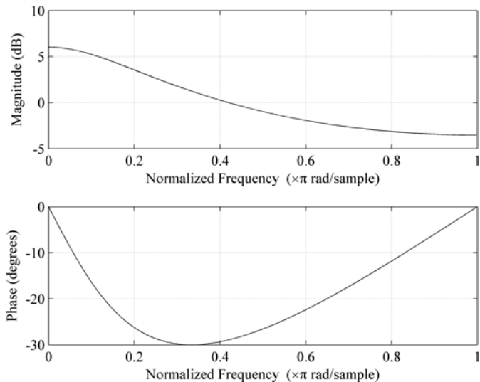
Fig. 4.7. Detailed computer-based frequency/phase response plots of y[n] = x[n] + 0.5 \cdot y[n - 1] . Top shows the magnitude response and bottom the phase response [in MATLAB ® : FREQZ(1, [1 -0.5]) ].
