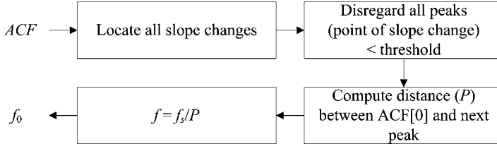
Fig. 5.9. Autocorrelation pitch computation.
