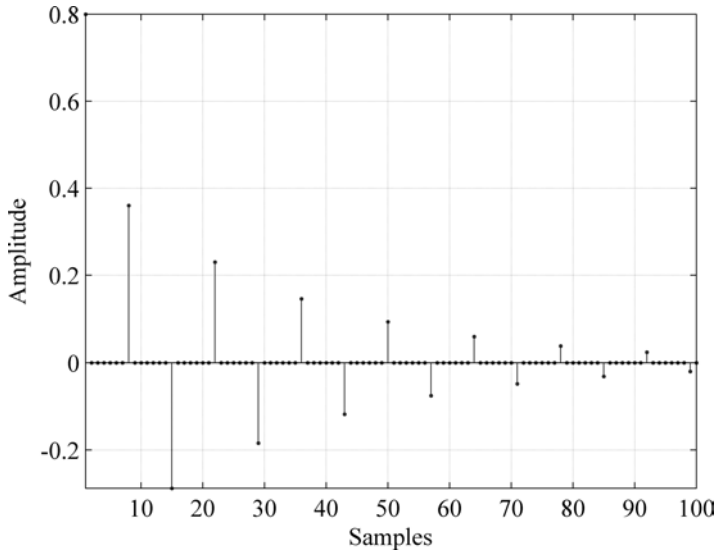
Fig. 3.41. All-pass filter N = 6 , \alpha = 0.8 .
