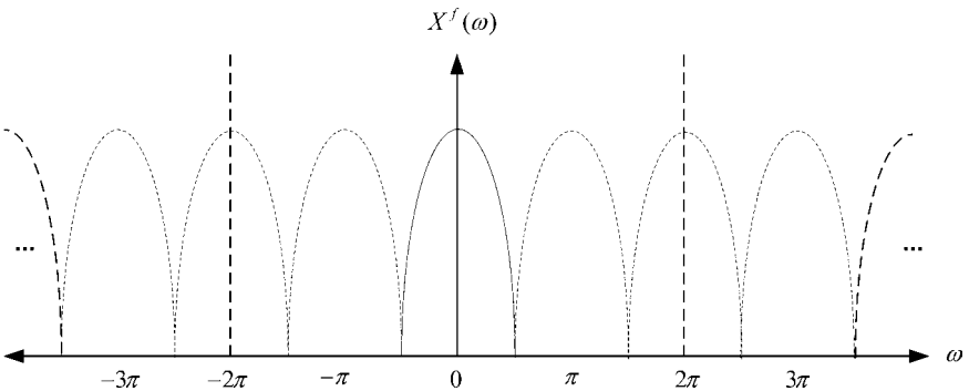
Fig. 8.4. Up-sampling by factor L = 2 .
