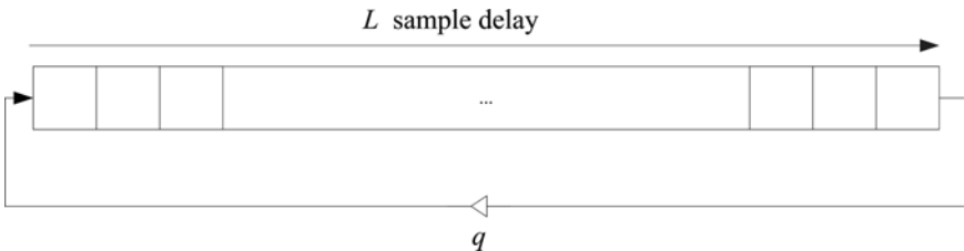
Fig. 3.18. Consolidated dampened plucked string.
