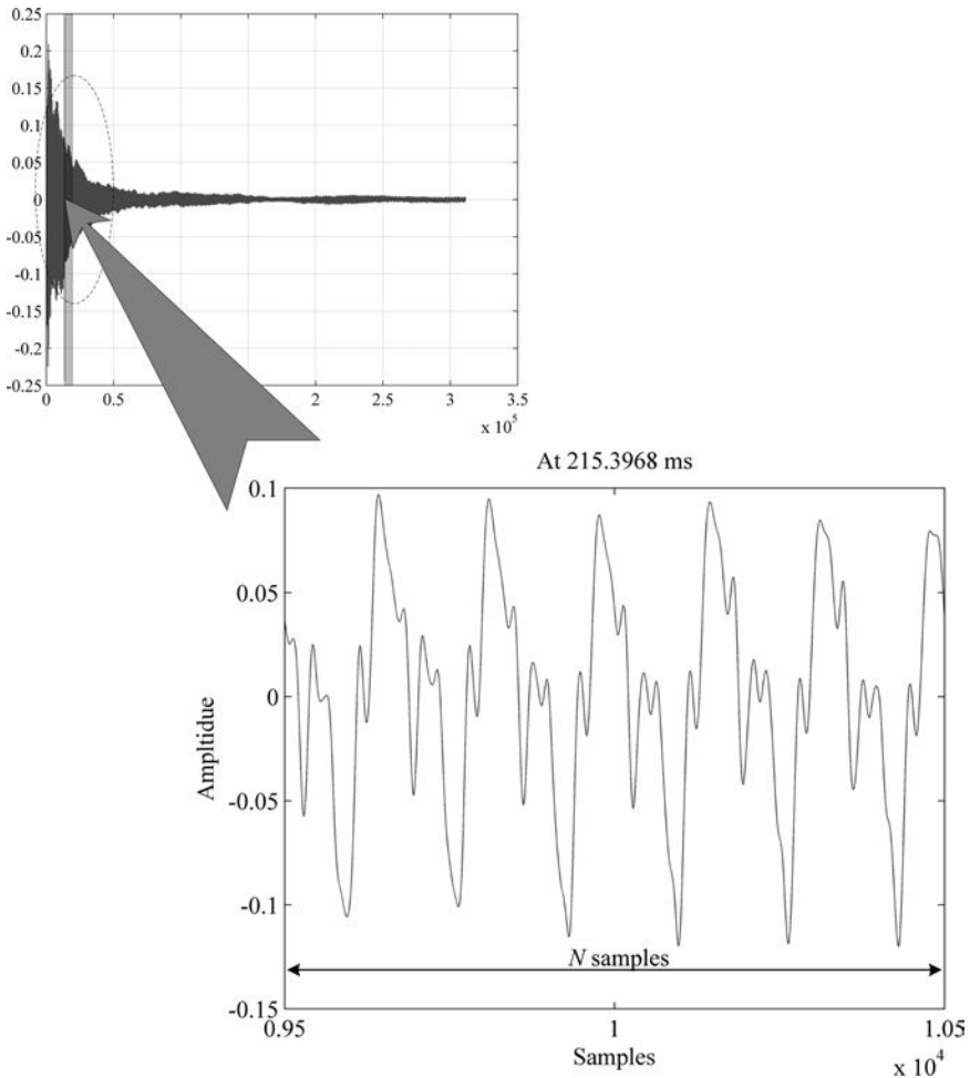
Fig. 4.2. Windowing of piano sample.
