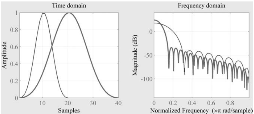
Fig. 9.11. Blackman window.
