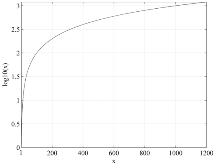
Fig. 2.3. Log function.
