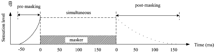
Fig. 3.5. Masking characteristics.
